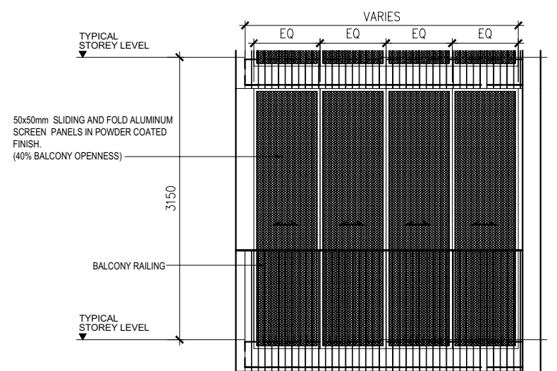
BALCONY / PES SCREEN - FRONT ELEVATION (External View)
